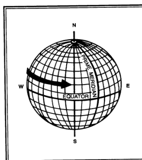
Figure 7-1. Rotation of the earth
